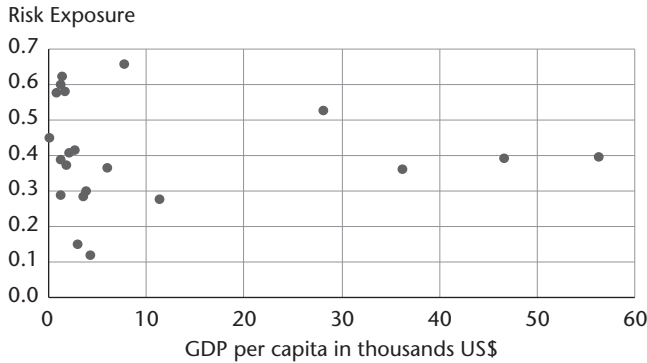
Figure 3.9 Annual mean PM2.5 Health Risk Exposure and GDP per capita in Asian countries/regions, 1990–2013
